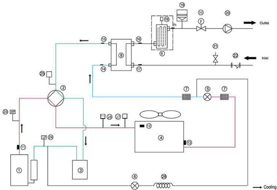
Figure 2-2.4: Cooling mode of 8/10/12/14/16kW
