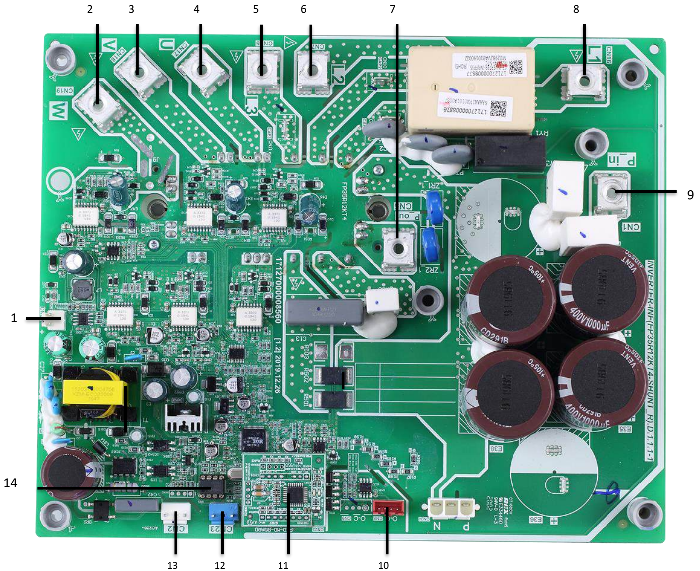
Figure 4-2.7: MHC-V12(14, 16)W/D2RN8-B outdoor unit inverter module
