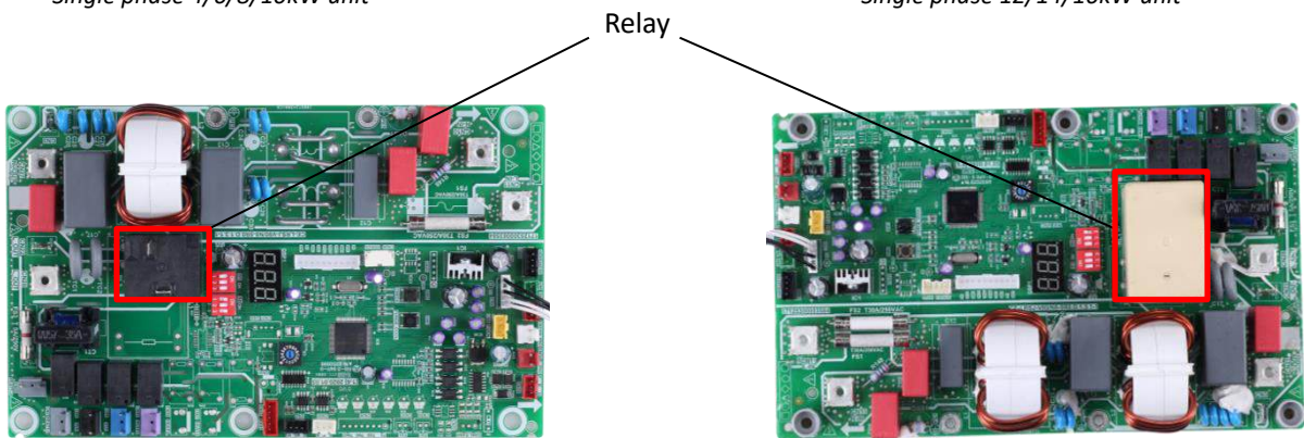
Figure 4-5.4: Relay location of main PCB for refrigerant system Single phase 4/6/8/10kW unit
