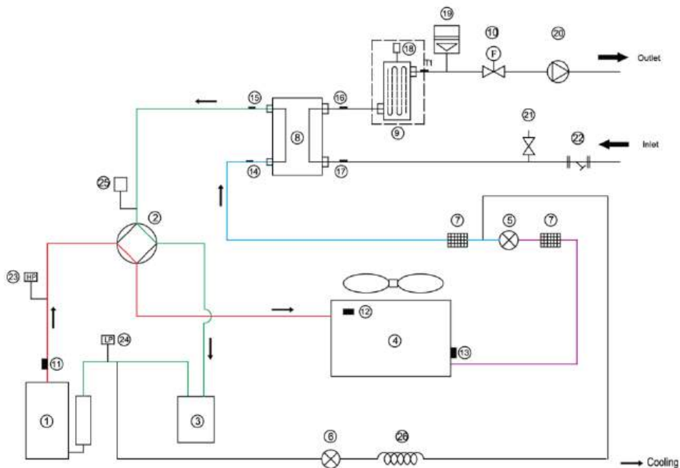
Figure 2-2.2: Cooling mode of 4/6kW
