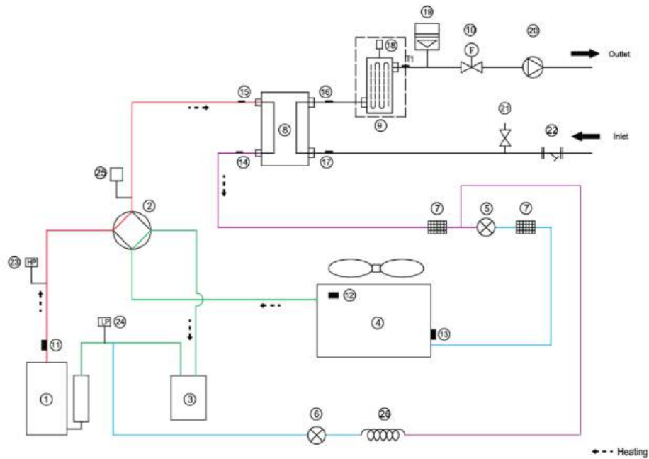
Figure 2-2.1: Heating mode of 4/6kW
