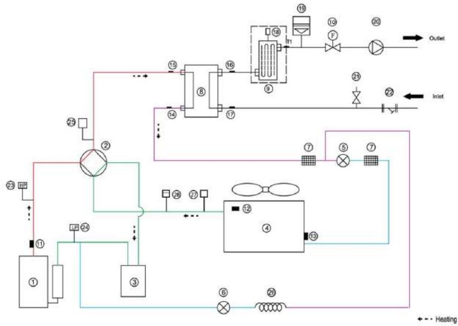
Figure 2-2.3: Heating mode of 8/10/12/14/16kW
