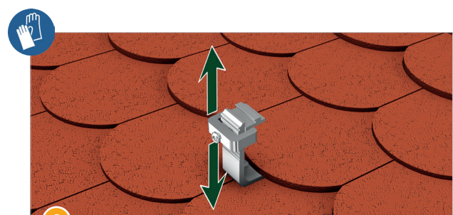
6 The clamp combination is adjustable in height by +/-25mm and is only screwed together with the rail.
